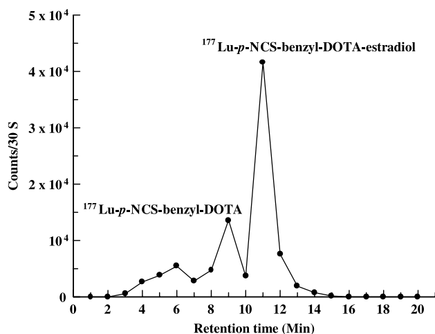
Figure 1. HPLC pattern of 177 Lu- p -NCS benzyl-DOTA-estradiol complex using water (A) and methanol (B) as mobile phase (0–4 min 90% A, 4–10 min 90% A to 10% A, 10–15 min 10% A to 90% A, 15–20 min 90% A).
